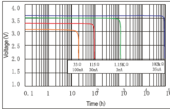
Typical Discharge Characteristics at 25°C
