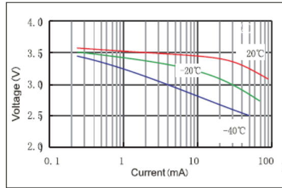
Voltage and Temperature Curve
