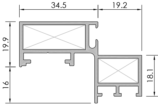
Cam Paneli
