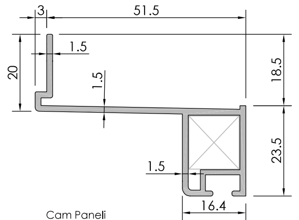
Cam Paneli
