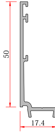
Sill Profile - Pervaz Profili
