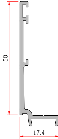
Corner Cleat - İlave Kulak
