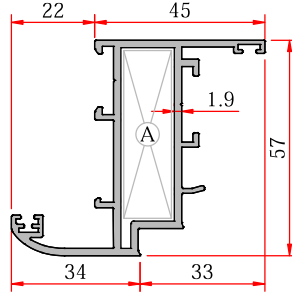
Narrow Vent - Dar Kanat
