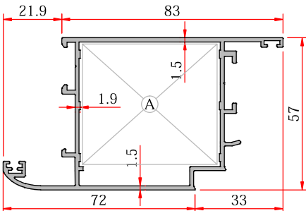
Narrow Vent - Dar Kanat
