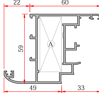
Narrow Vent - Dar Kanat
