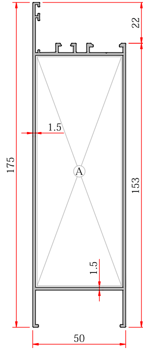
Wide Sill Profile - Geniş Etek Profili
