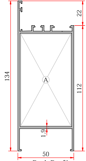
Sill Profile - Etek Profili
