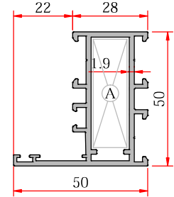
Narrow Vent - Dar Kasa
