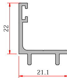
Corner Cleat - İlave Kulak
