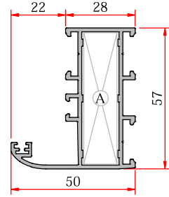
Narrow Frame - Dar Kasa
