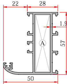
Narrow Vent - Dar Kasa
