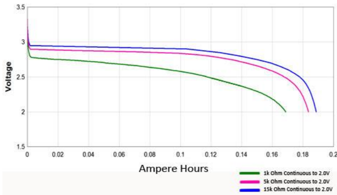
Continuous Discharge Characteristics
