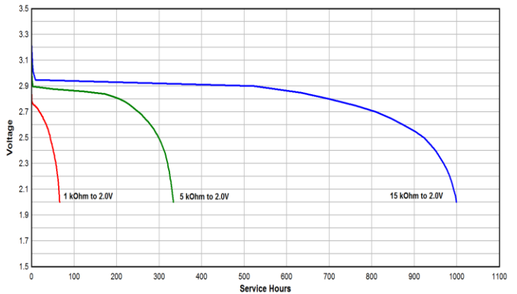
Continuous Discharge - Service Life
