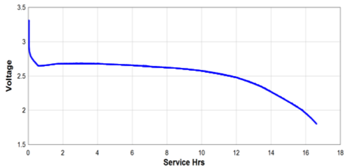
ANSI Key Fob Test 10 mA 5s/m, 24hd 1.8 New
