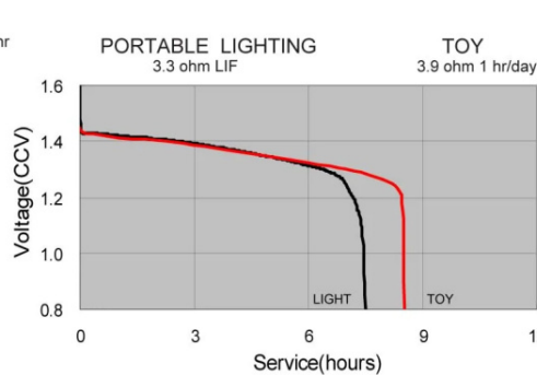
Application Tests(23±2°C)
