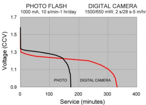
Application Tests(23±2°C)
