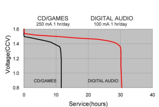
Application Tests(23±2°C)
