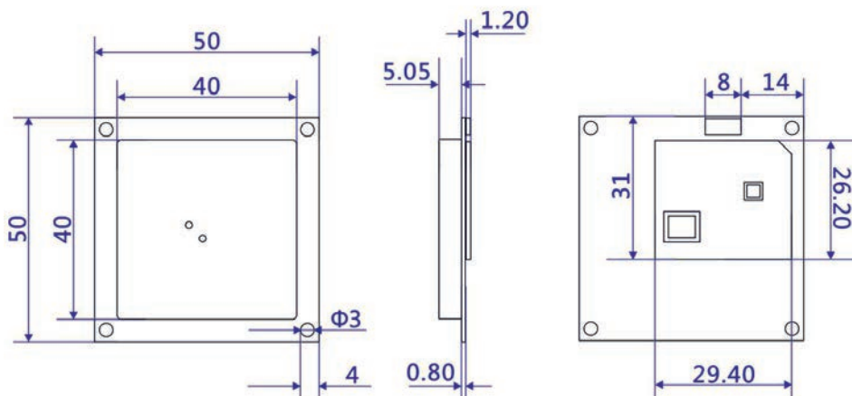
Figure 3-1 RX3 Dimensions
