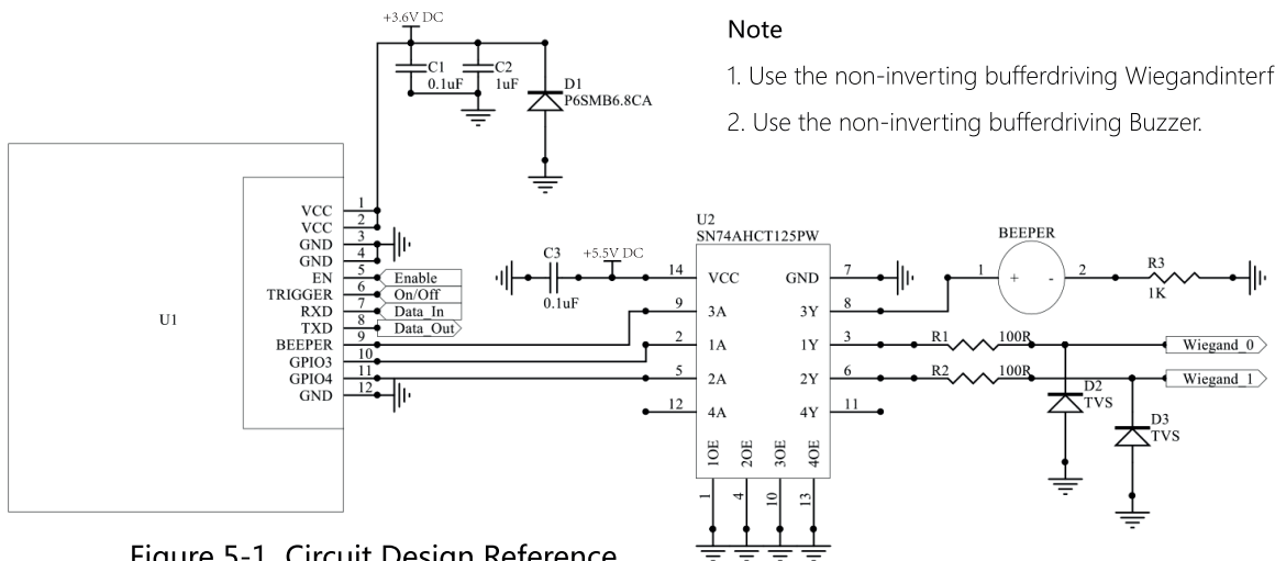
Figure 5-1 Circuit Design Reference
