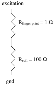
Figure 3a: Simplified circuit of contaminated probe in low EC (high resistance) soil. R_{\text{total}} = 101 \Omega , fingerprint causes 1% error.
