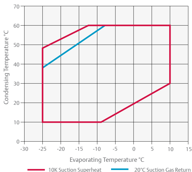
Operating Envelope ZS* KA R448A/R449A
