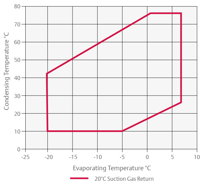
Operating Envelope ZS* KA R134a
