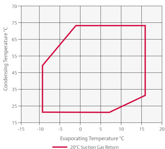
Operating Envelope ZB* KA R134a
