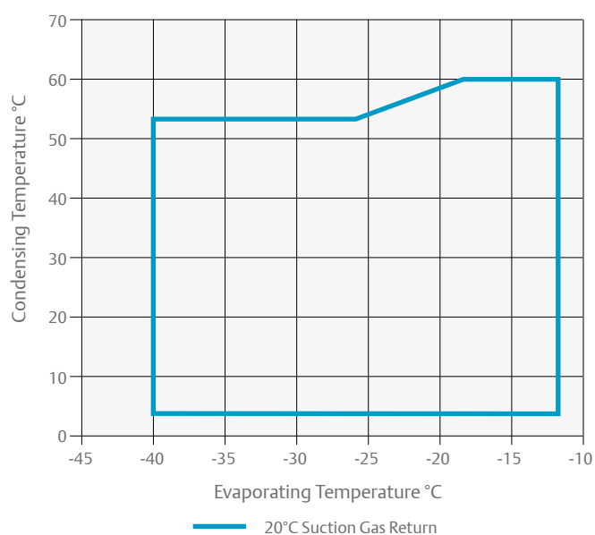
Operating Envelope ZF* KA R448A/R449A
