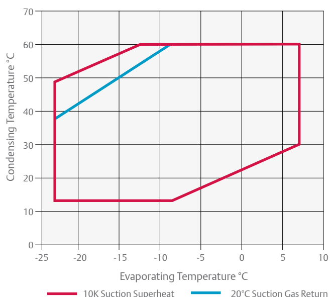
Operating Envelope ZB* KA R448A/R449A
