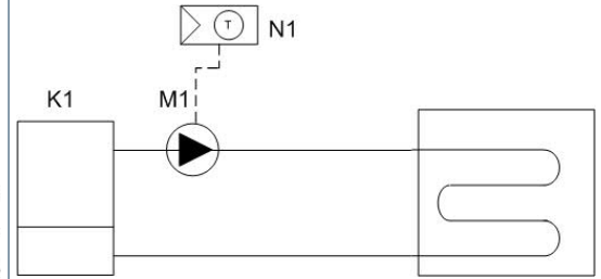
Floor heating with pump
