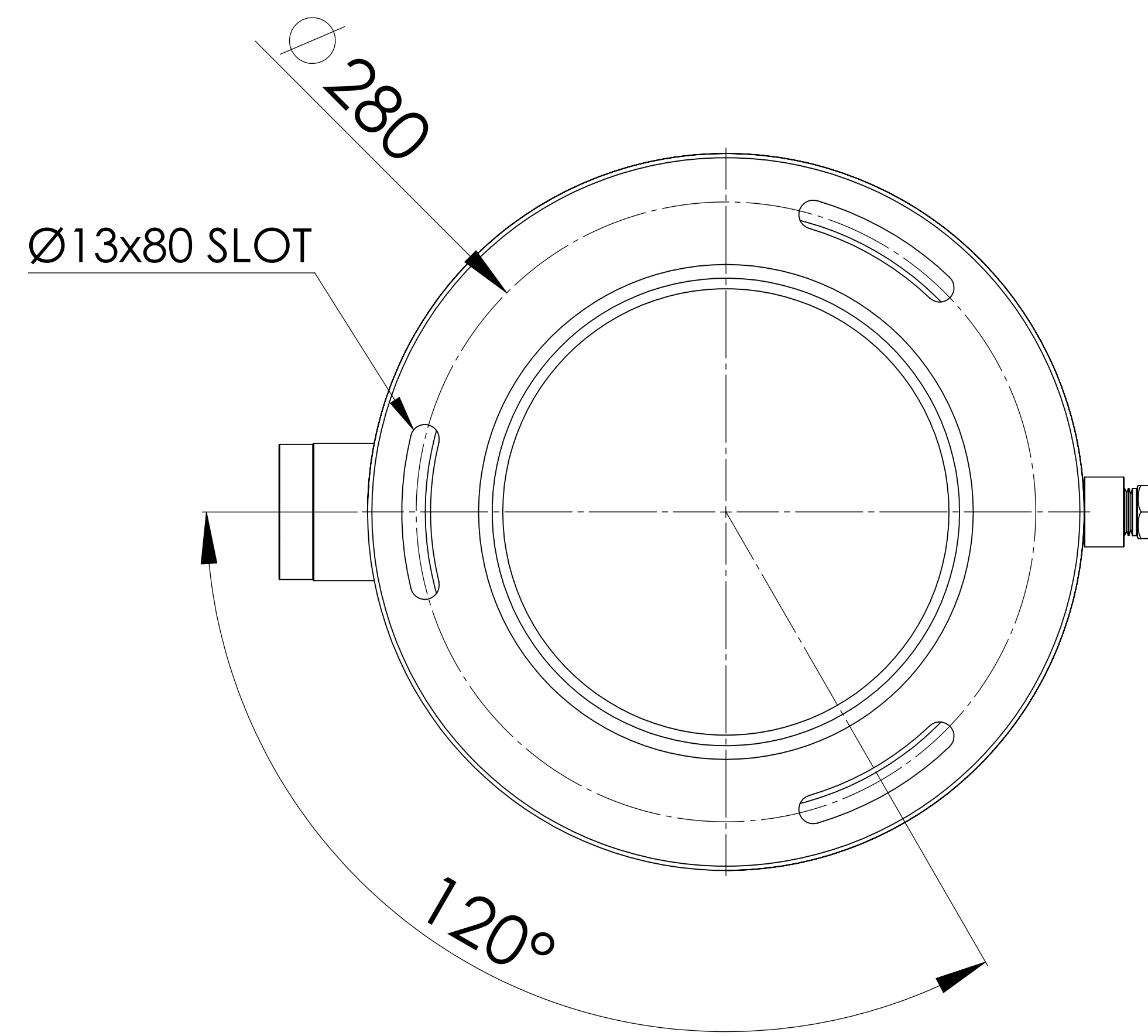
BOTTOM VIEW
