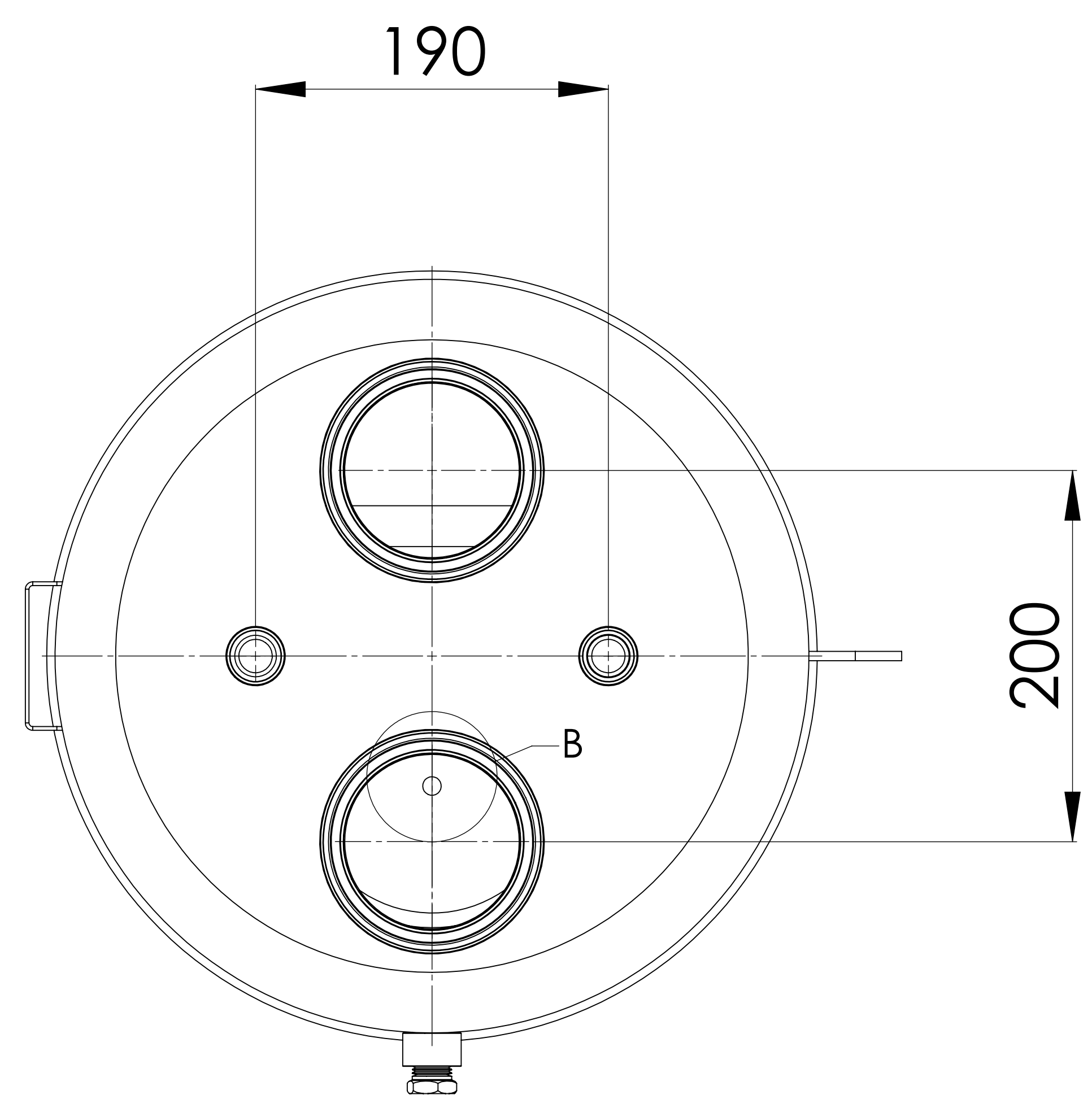
TOP VIEW
