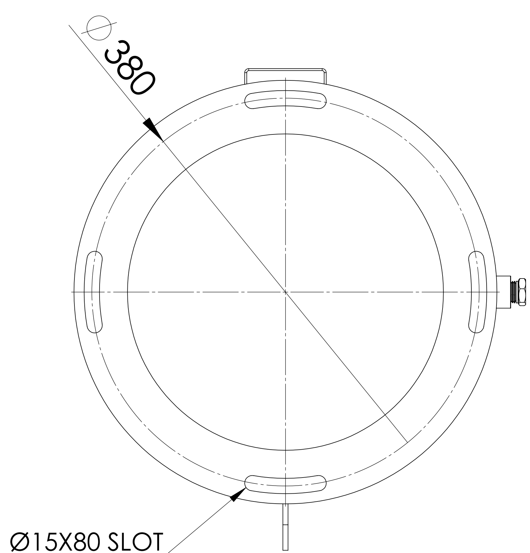
BOTTOM VIEW
