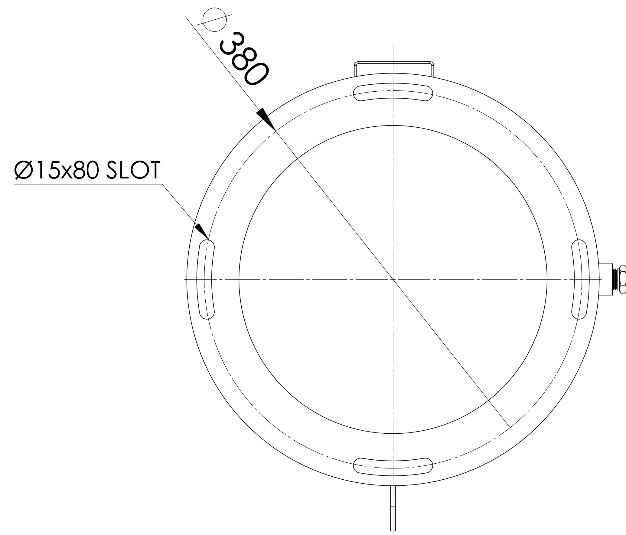
BOTTOM VIEW
