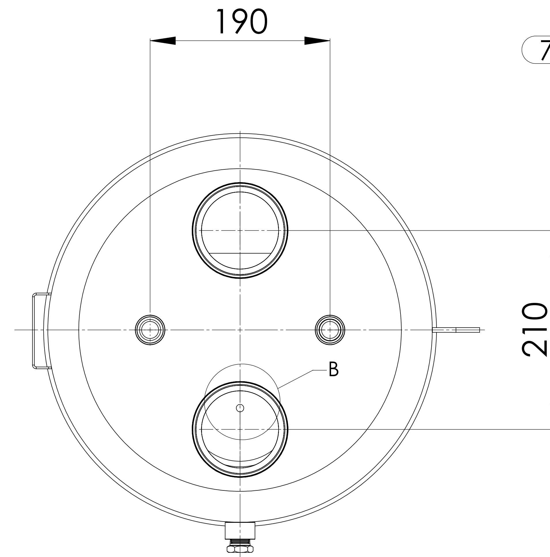
TOP VIEW
