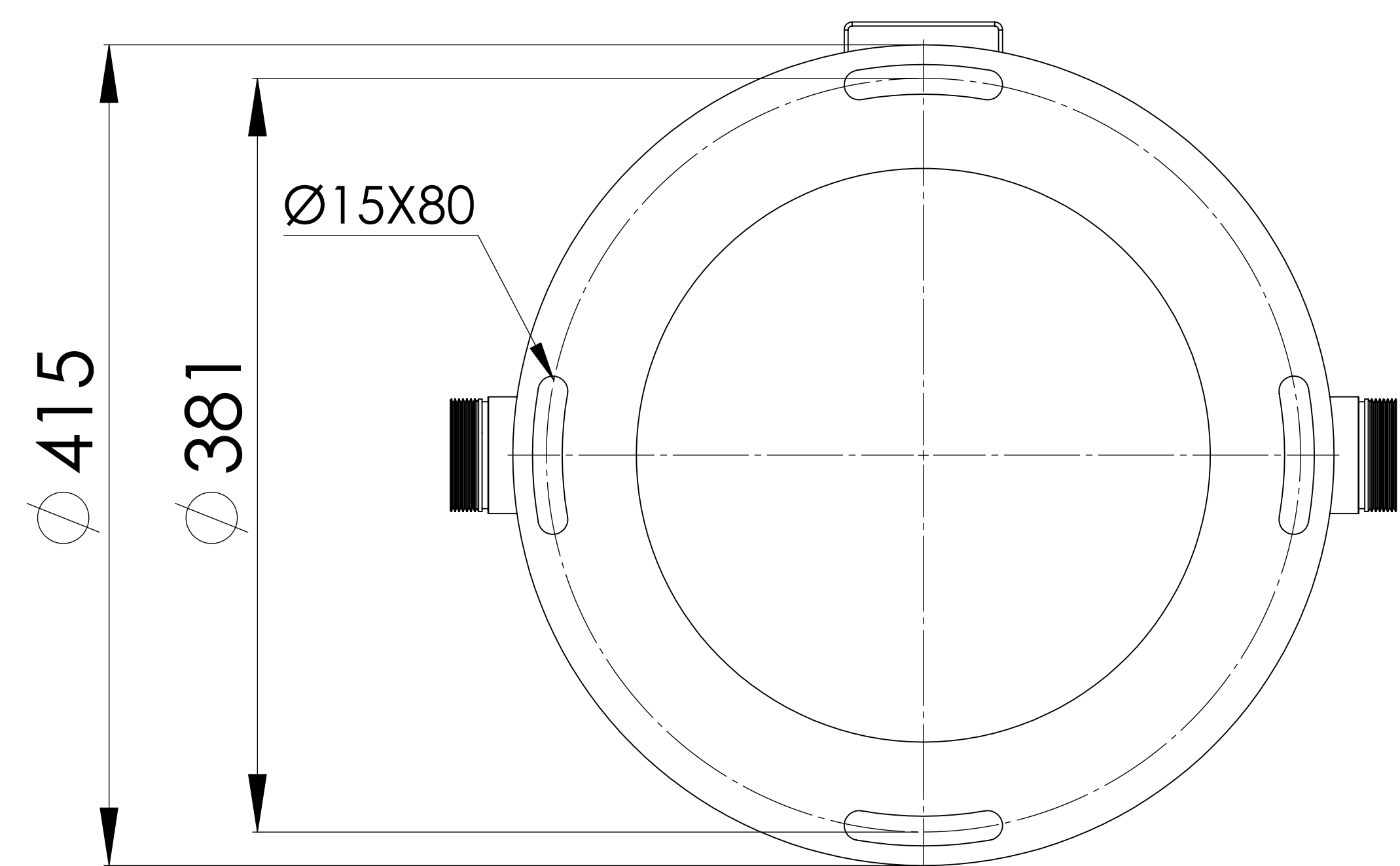
BOTTOM VIEW
