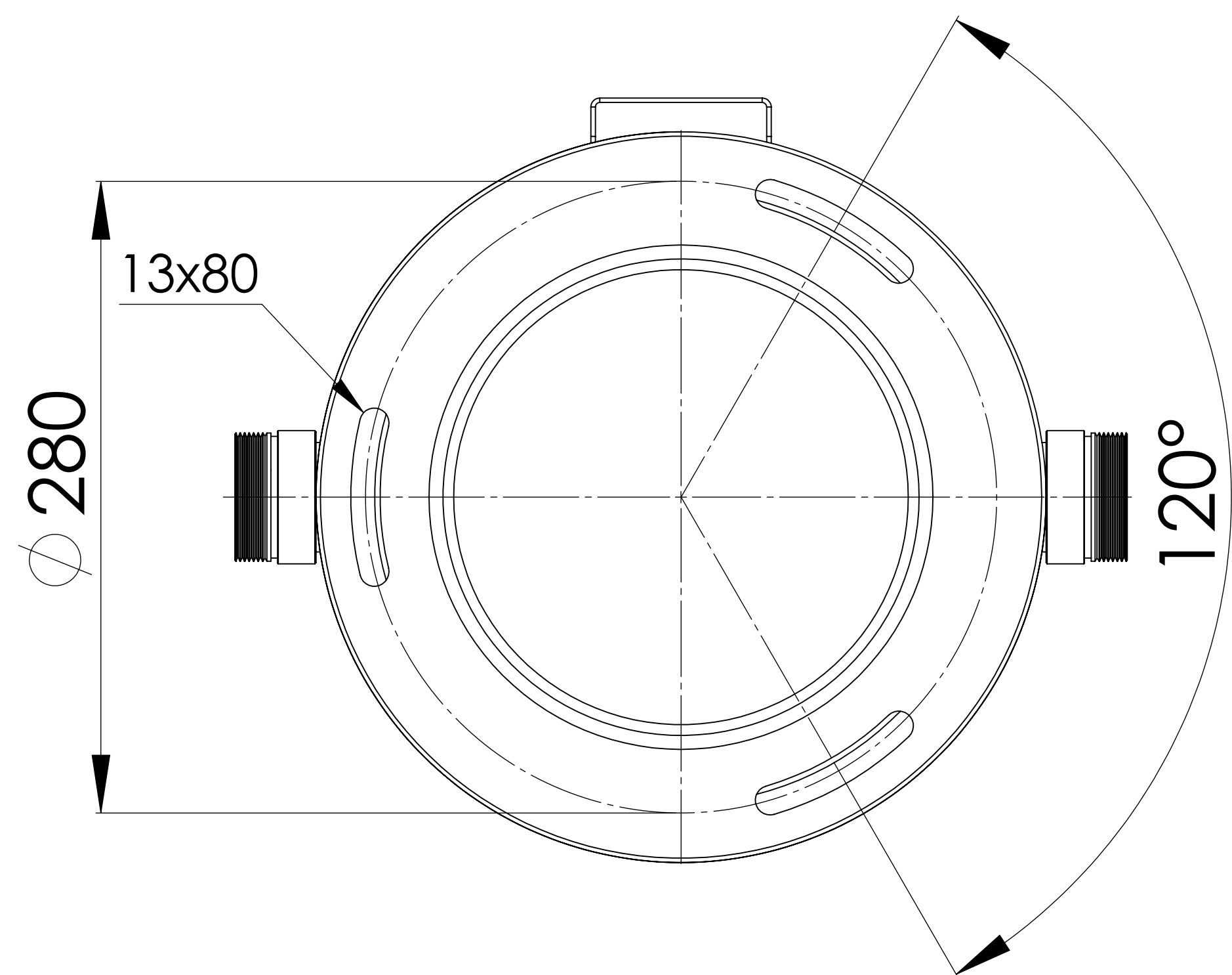
BOTTOM VIEW
