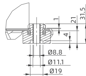
Mounting Feet
