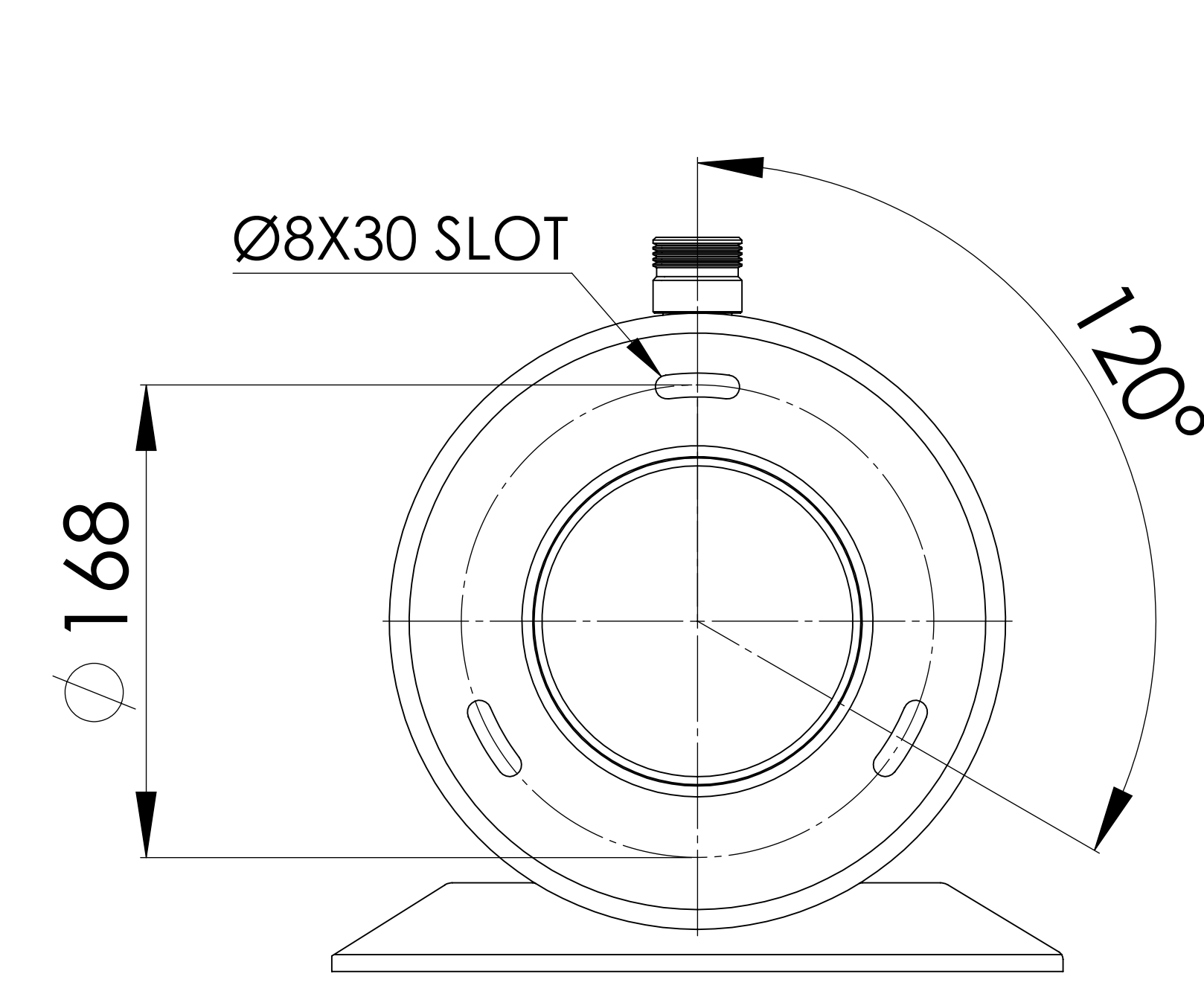
BOTTOM VIEW
