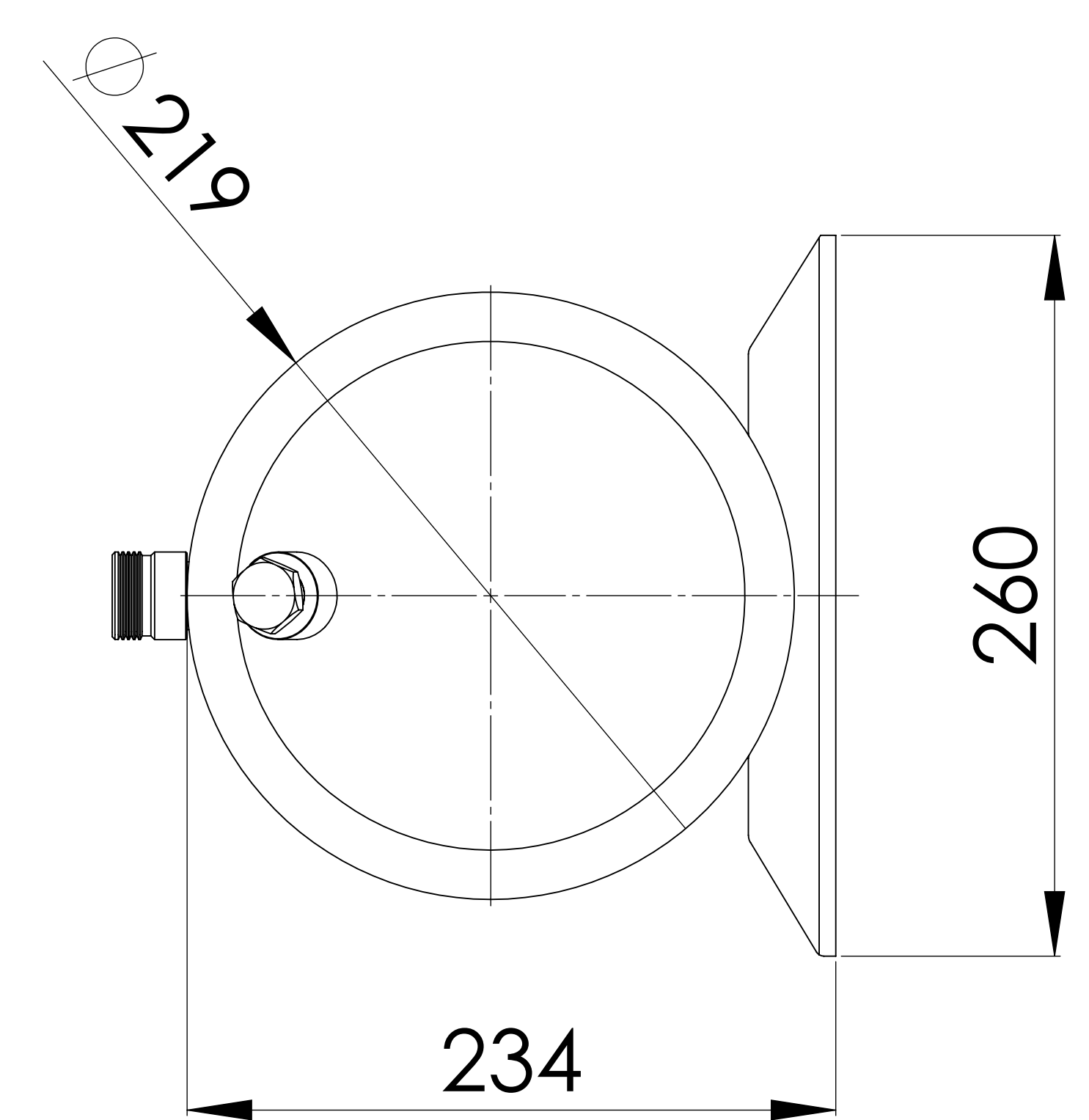
TOP VIEW
