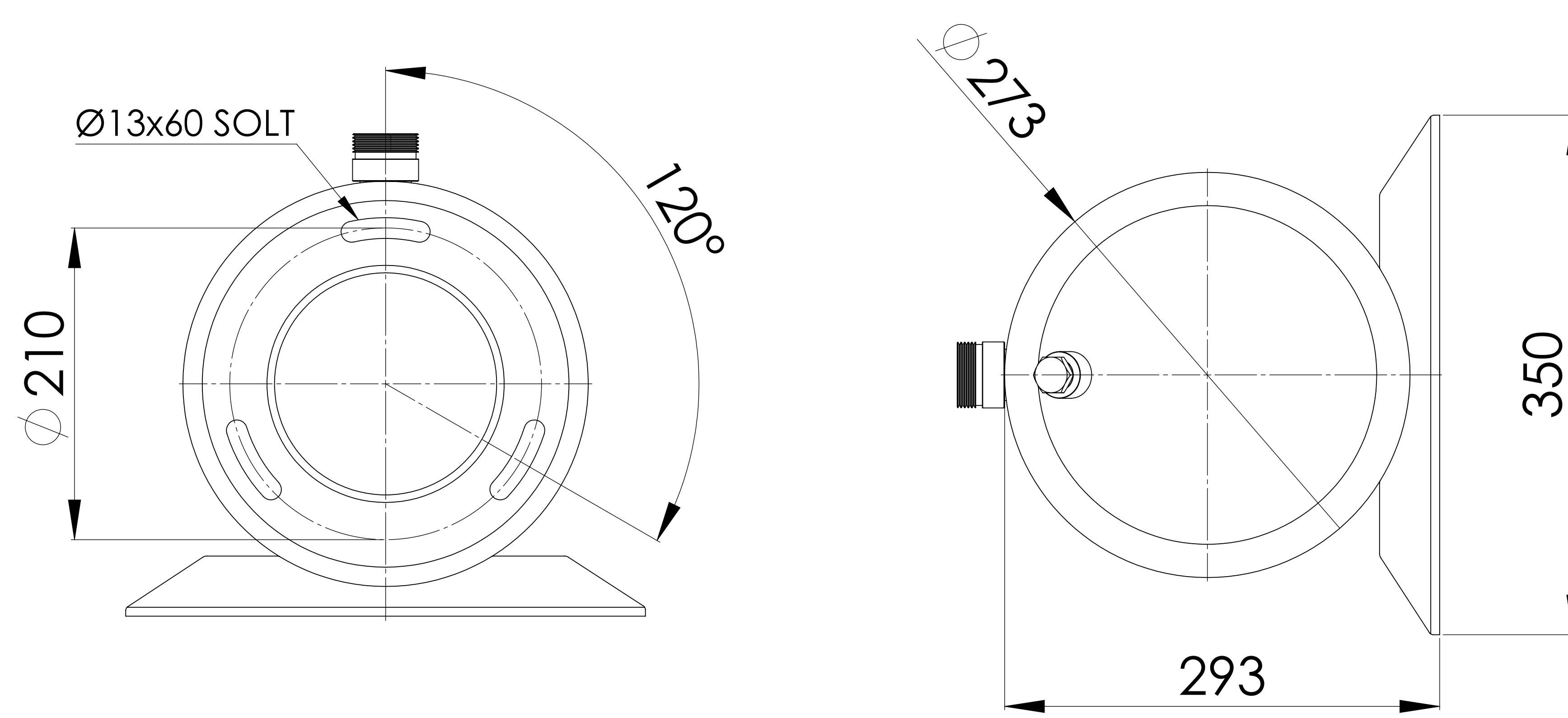
BOTTOM VIEW
