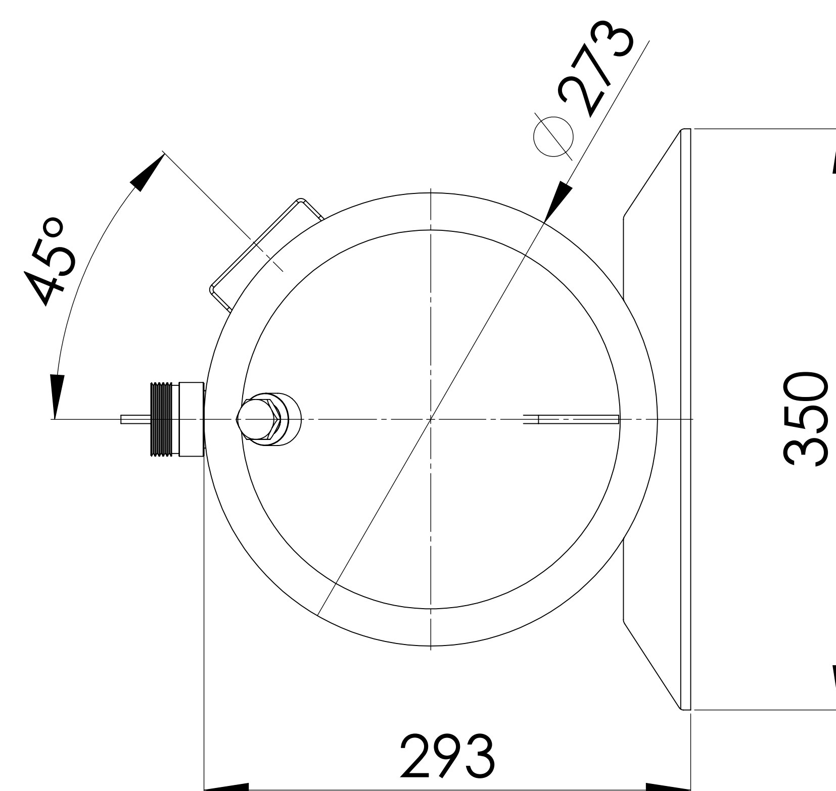
TOP VIEW
