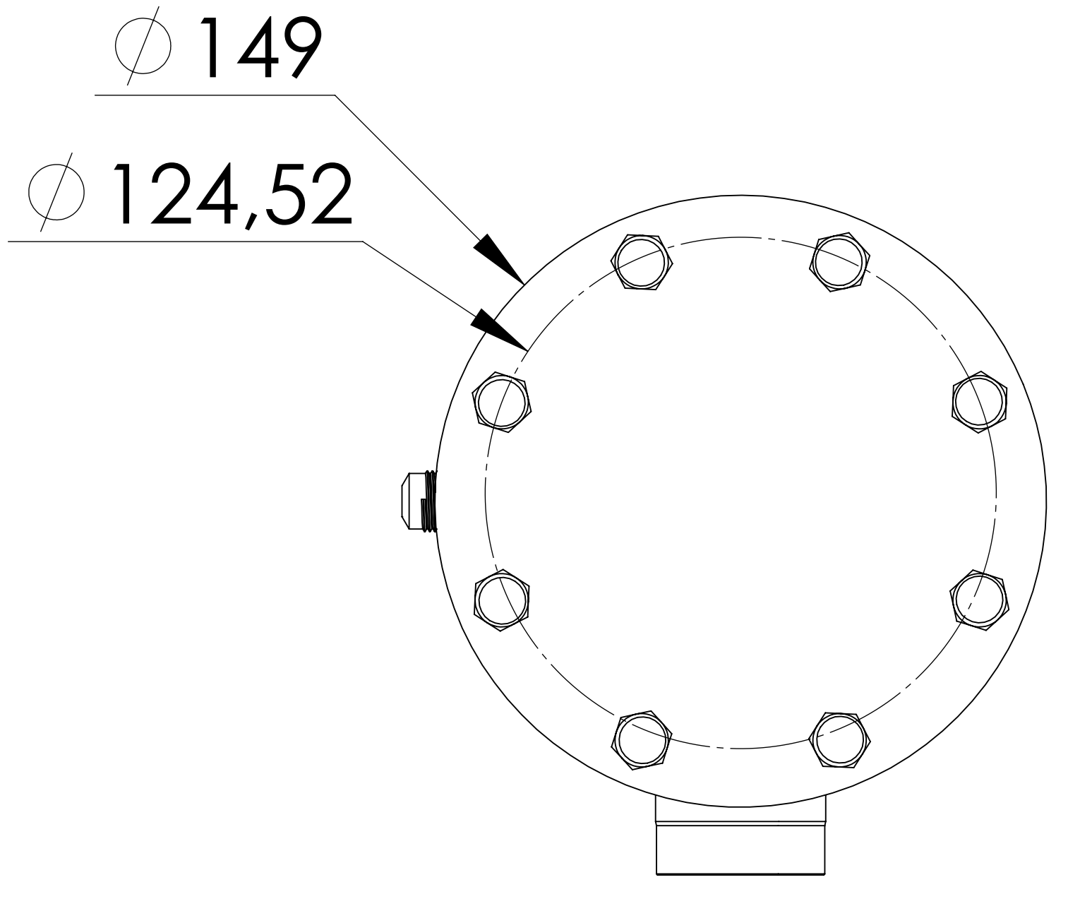
Top View
