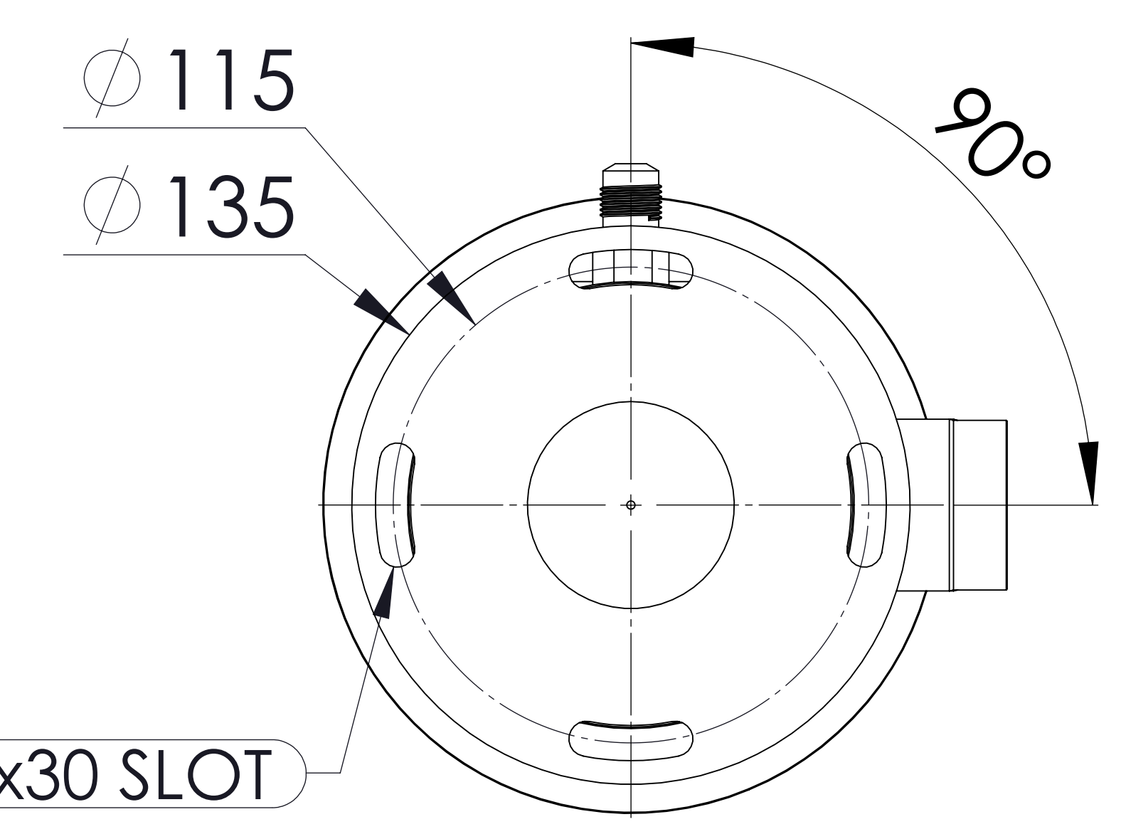
Bottom View
