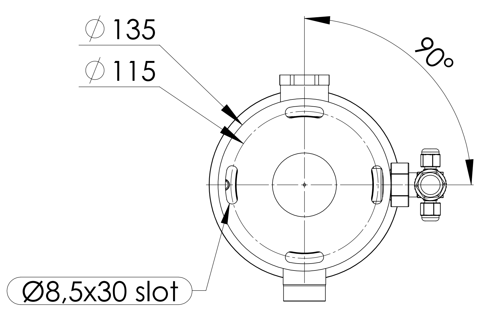
Bottom View
