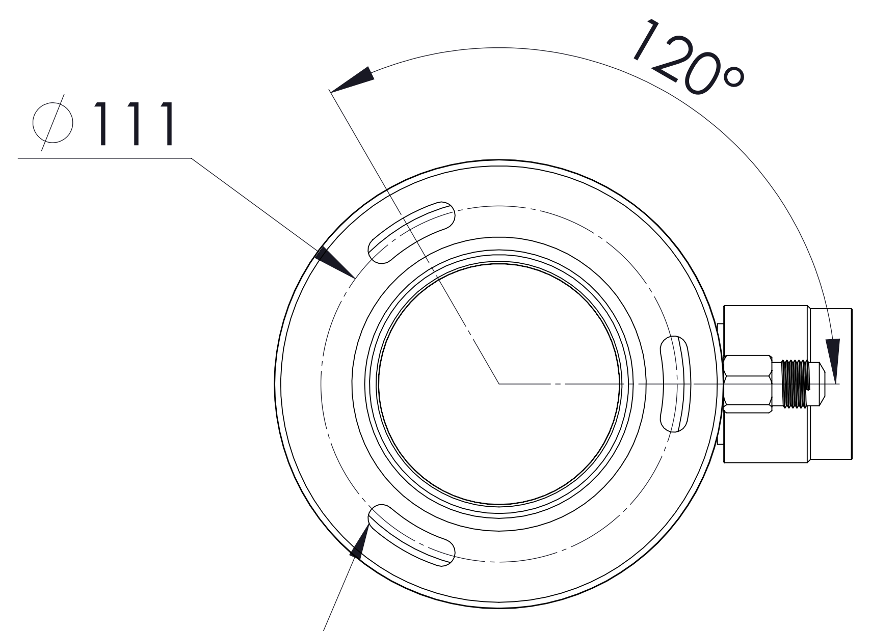
Bottom View
