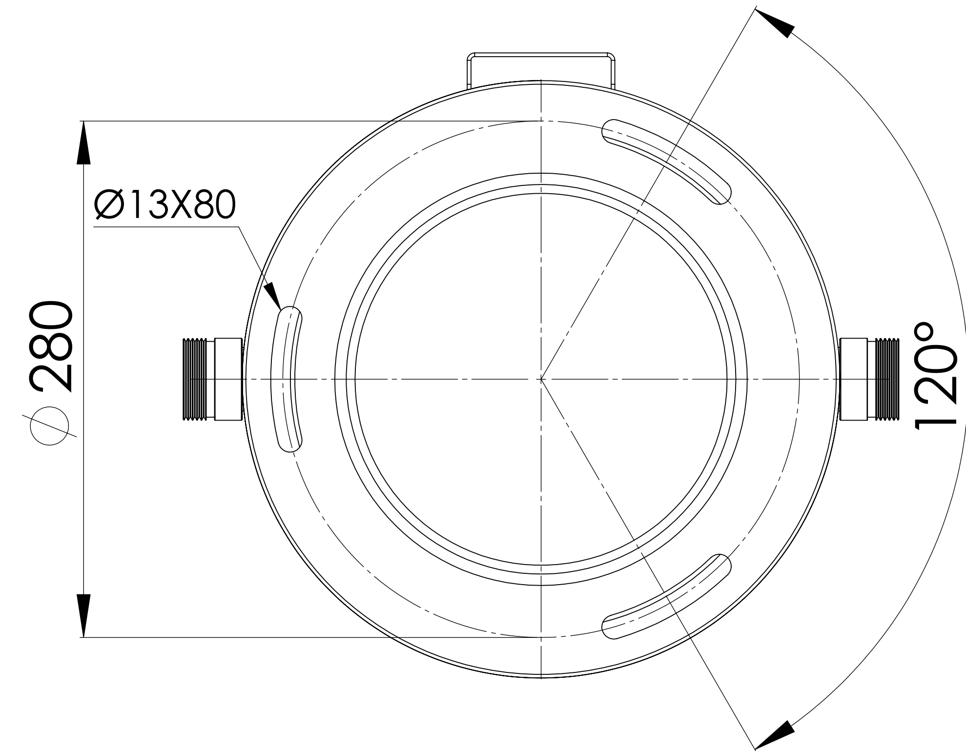
BOTTOM VIEW
