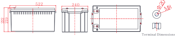
Terminal Dimensions
