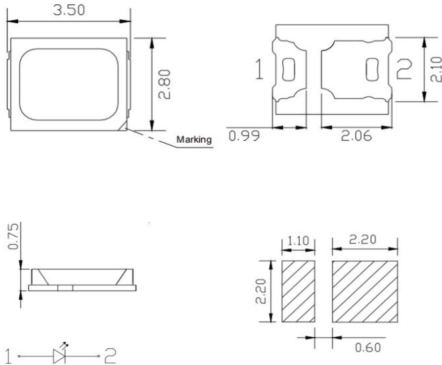
Soldering Pad Dimension
