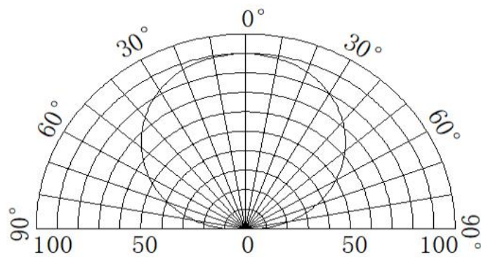
Intensity Distribution Diagram
