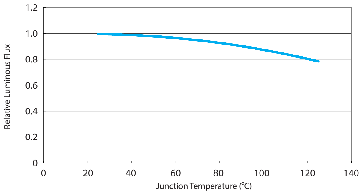
Relative Luminous Flux vs. Junction Temperature
