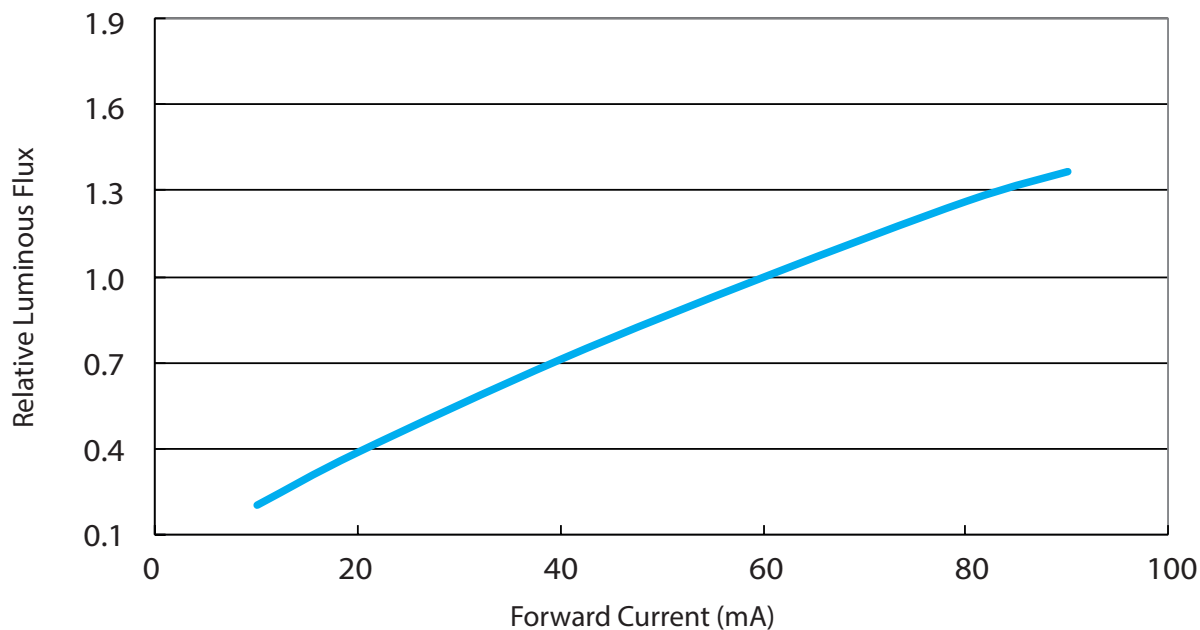
Relative Luminous Flux vs. Forward Current
