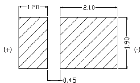
Solder Pad
