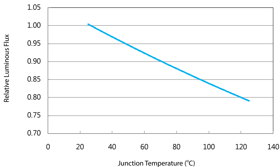
Relative Luminous Flux vs. Junction Temperature
