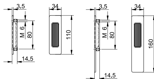
TECHNICAL DRAWING
