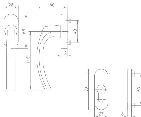
TECHNICAL DRAWING
