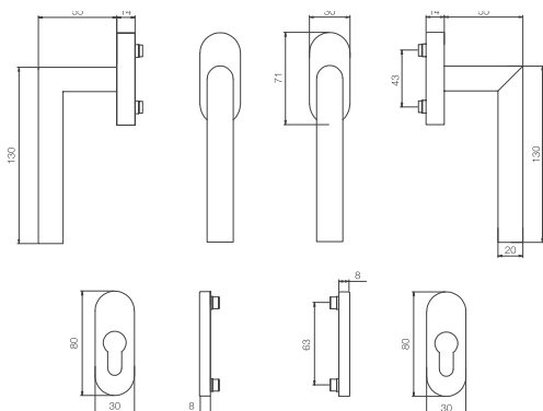
TECHNICAL DRAWING
