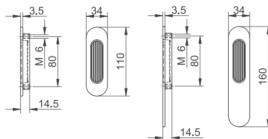
TECHNICAL DRAWING
