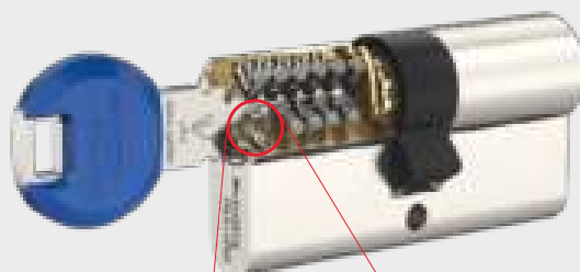
The security elements in the locking cylinder are matched to the moving active element in the key.
