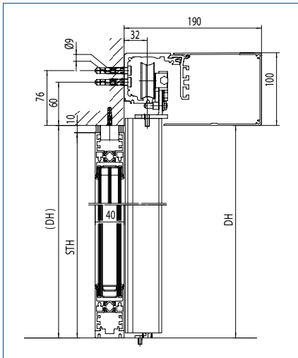
Drive length corresponding to or smaller than clear installation width
