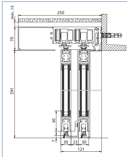
Drawing no. 70487-ep01
