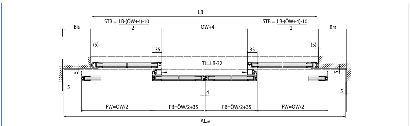
2-leaf, mounting within reveal, adjustable floor guide
