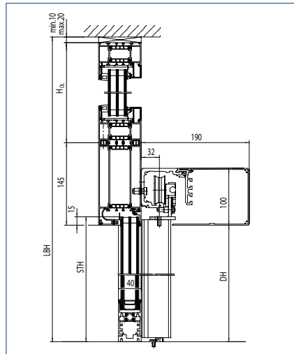
Vertical section side screen
