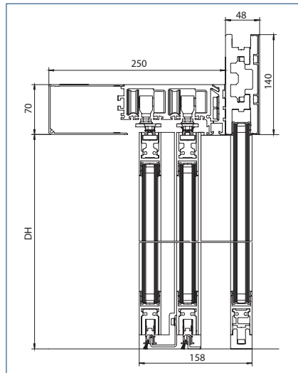
High girder section
