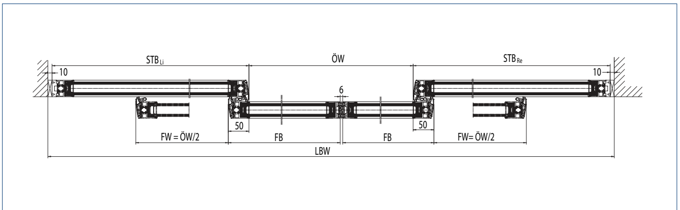
Drive length greater than clear installation width
