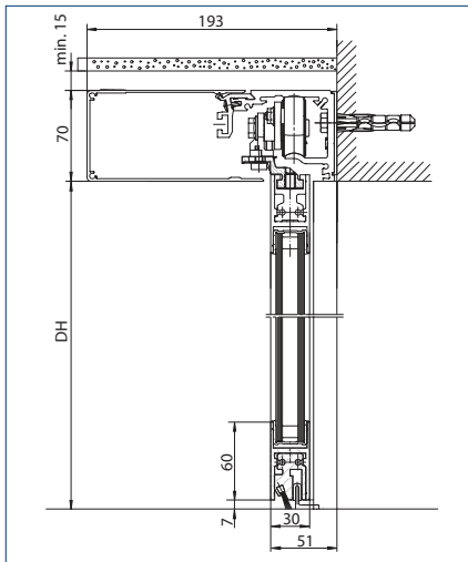
Drawing no. 70511-ep01
