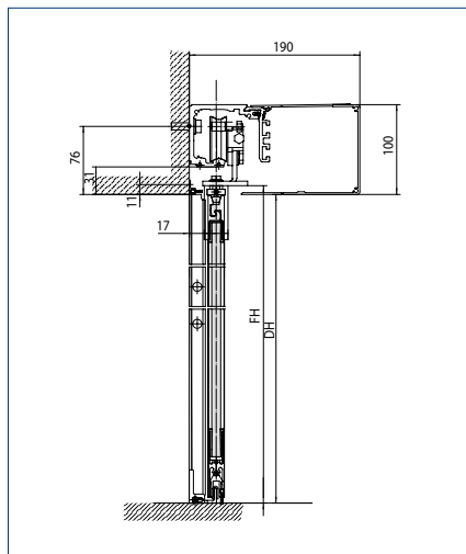
Drawing no. 70518–ep03 / 70518–ep04
