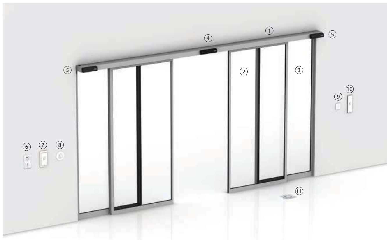
1 = Sliding door drive | 2 = Moving leaf | 3 = Side screen | 4 = Combined detector | 5 = Active infrared detector | 6 = Programme switch with key switch | 7 = Plastic elbow switch | 8 = LED sensor switch glass | 9 = Non-contact proximity switch | 10 = Elbow switch | 11 = LED sensor foot switch
