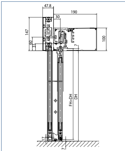
2-leaf, mounting within reveal, angled floor guide, protective leaf
