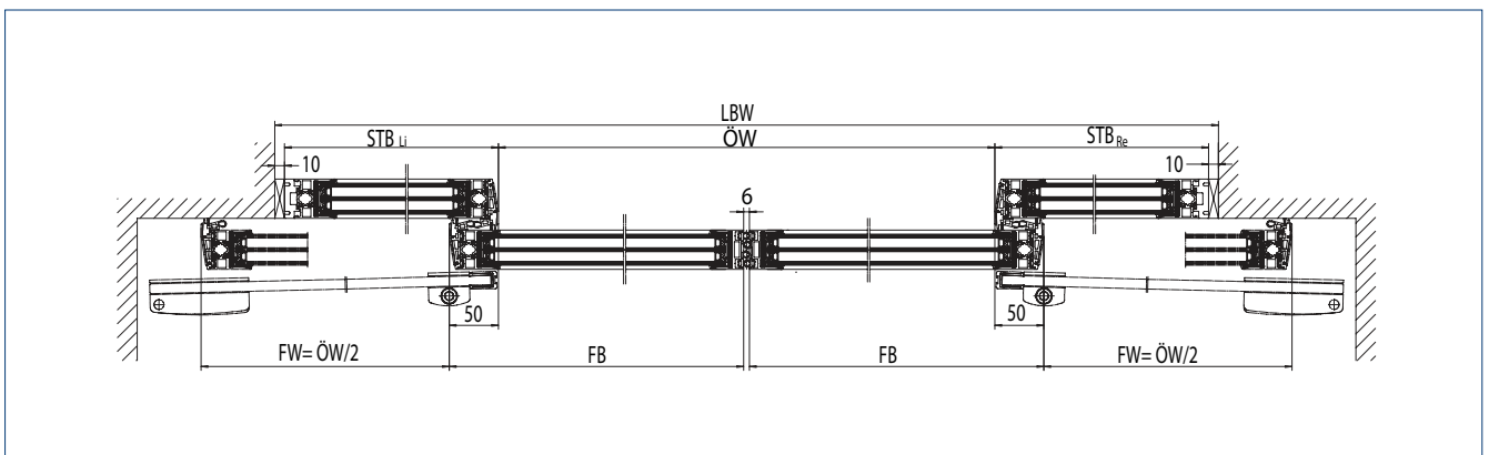
Drive length greater than clear installation width
