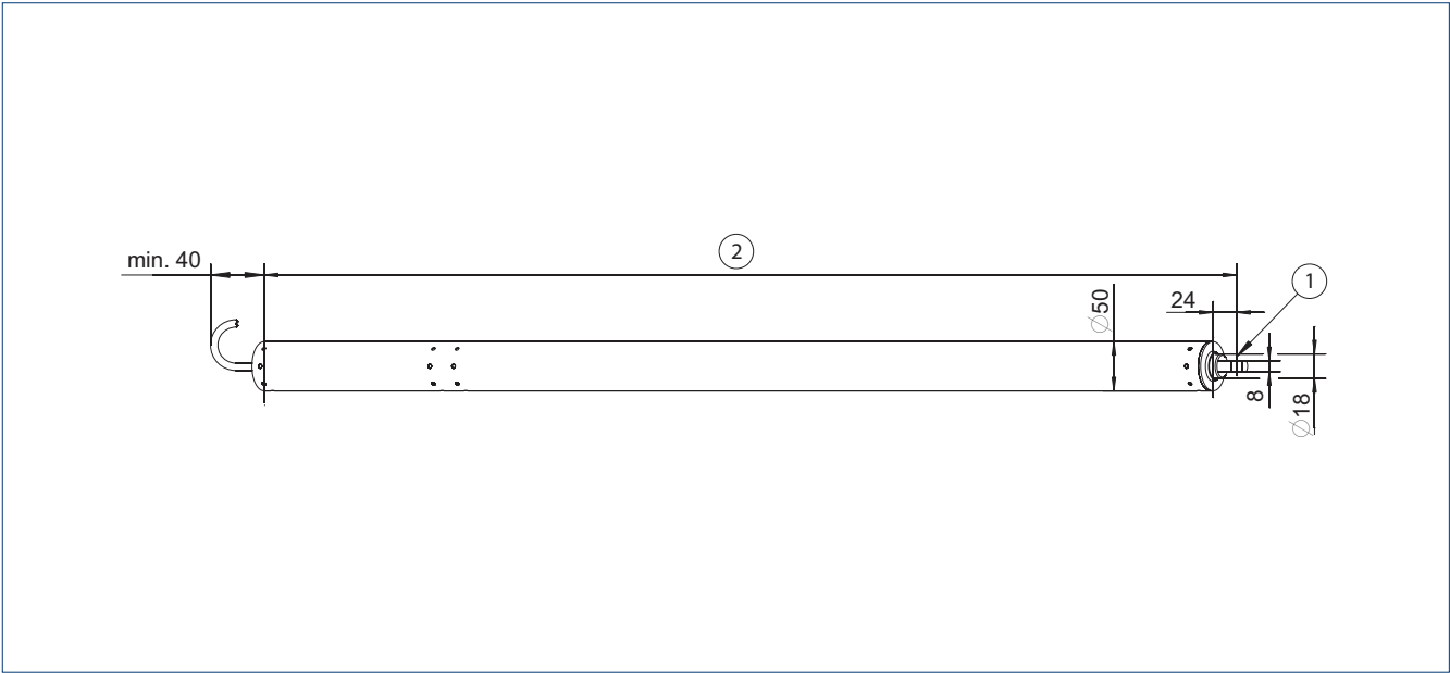
1 = Ø 6 mm with bearing bush, Ø 8 mm without bearing bush | 2 = approx. 465 mm + stroke
