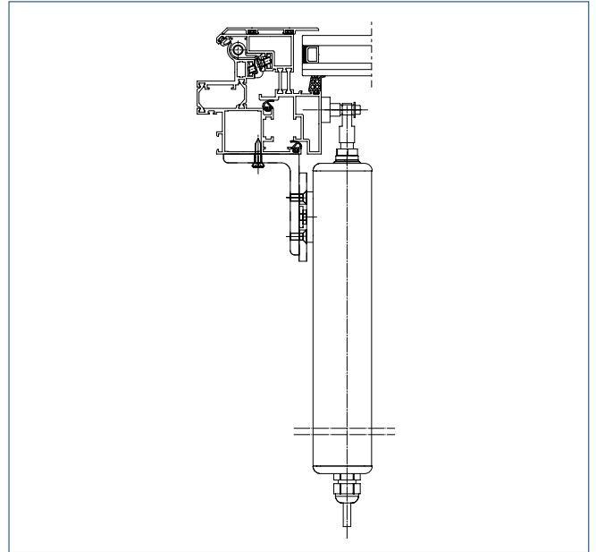
Leaf bracket E 1500 NSK W-HU (ID no. 136187) | Rotating bracket E 250 NT NSK / E 350 N, incl. bracket mount E 250 and eye bolt ø 8 mm (ID no. 138367)
