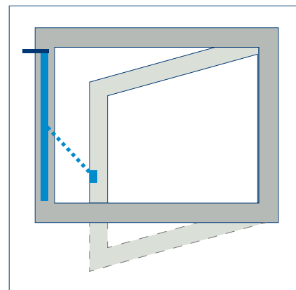
Side-hung leaf DIN L OUTWARD opening (drive cannot be swivelled) Cable outlet always upwards.
