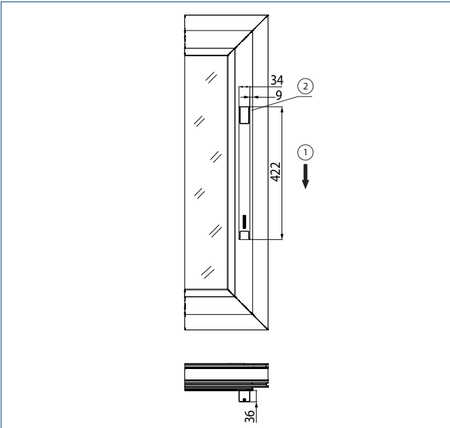
Space needed for leaf installation
