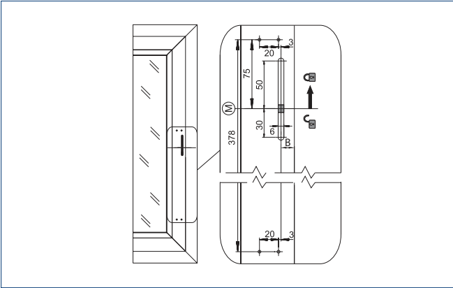
Installation dimensions leaf installation
