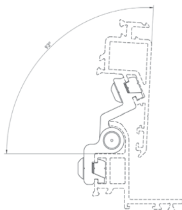
MAXIMUM OPENING ANGLE
